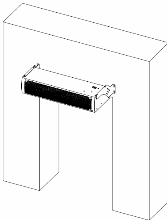
Standard mounting
