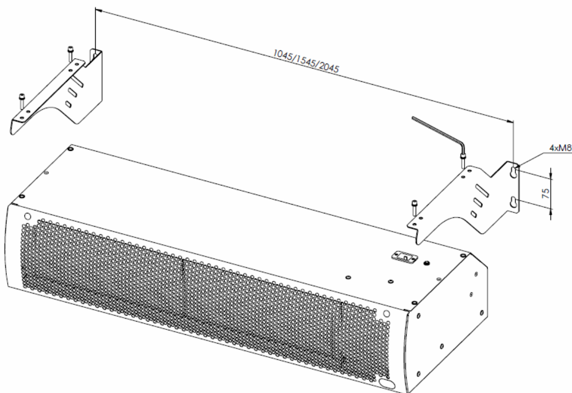
Drilling spacing and recommended mounting
